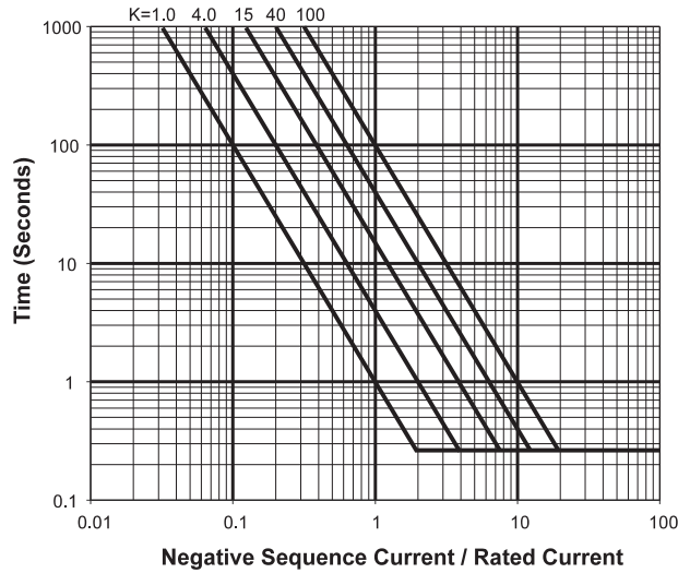
Figure 4-3: NEGATIVE SEQUENCE INVERSE TIME CURVES
