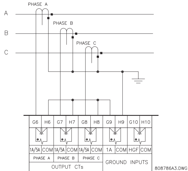
Figure 2-12: RESIDUAL GROUND CT CONNECTION
