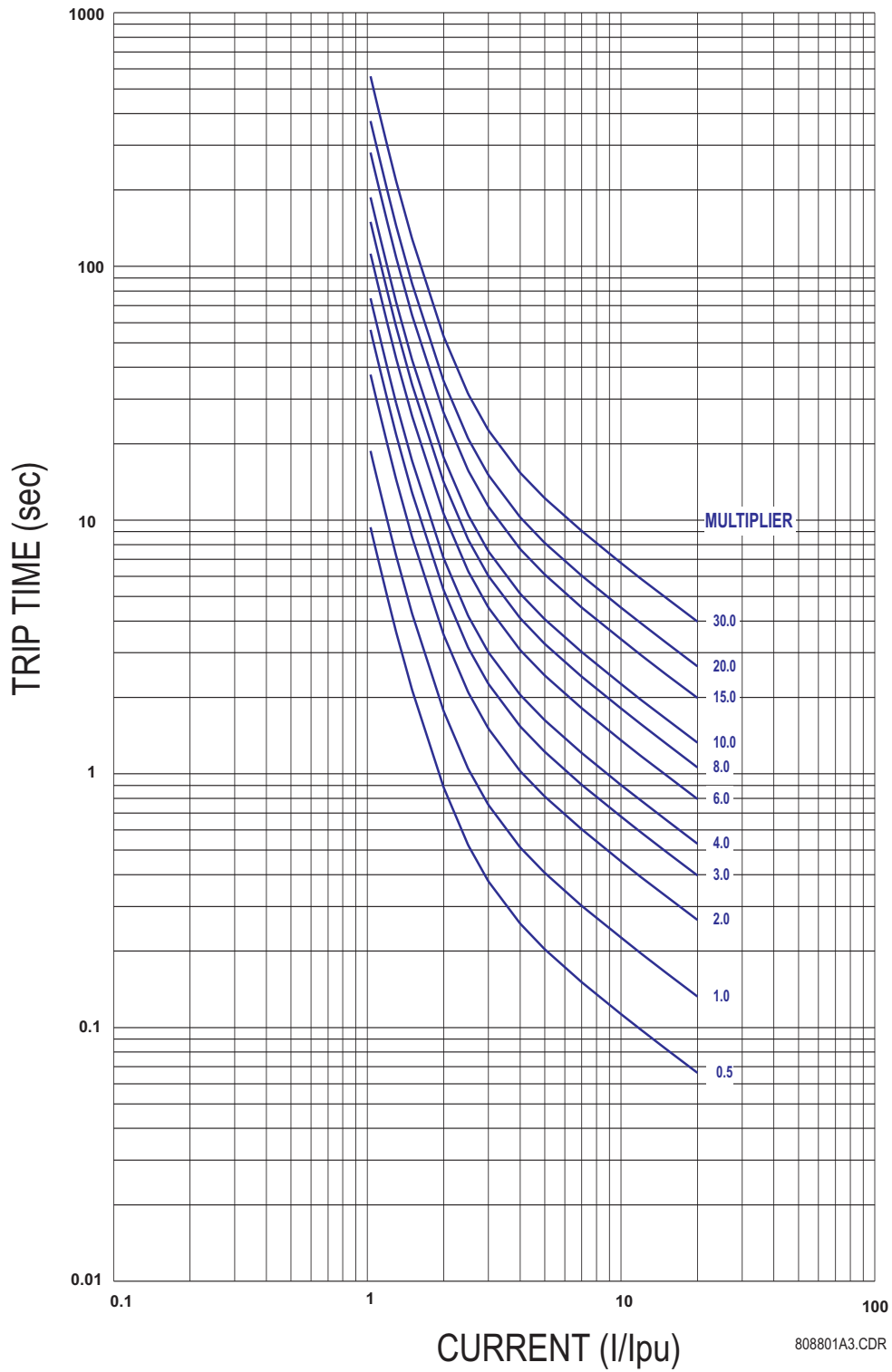
Figure C-2: ANSI NORMALLY INVERSE CURVE
