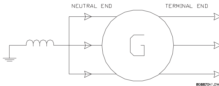
Figure 7-3: PHASE DIFFERENTIAL
