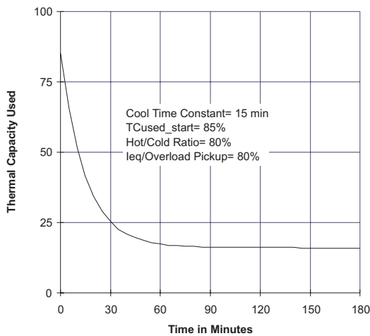
Thermal Model Cooling, 80% Load
