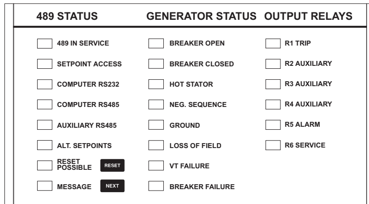
Figure 3-3: 489 LED INDICATORS
