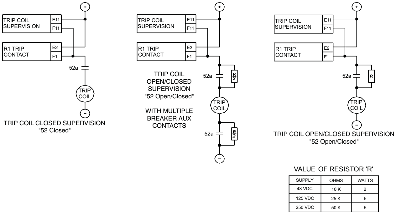
Figure 4-19: TRIP COIL SUPERVISION
