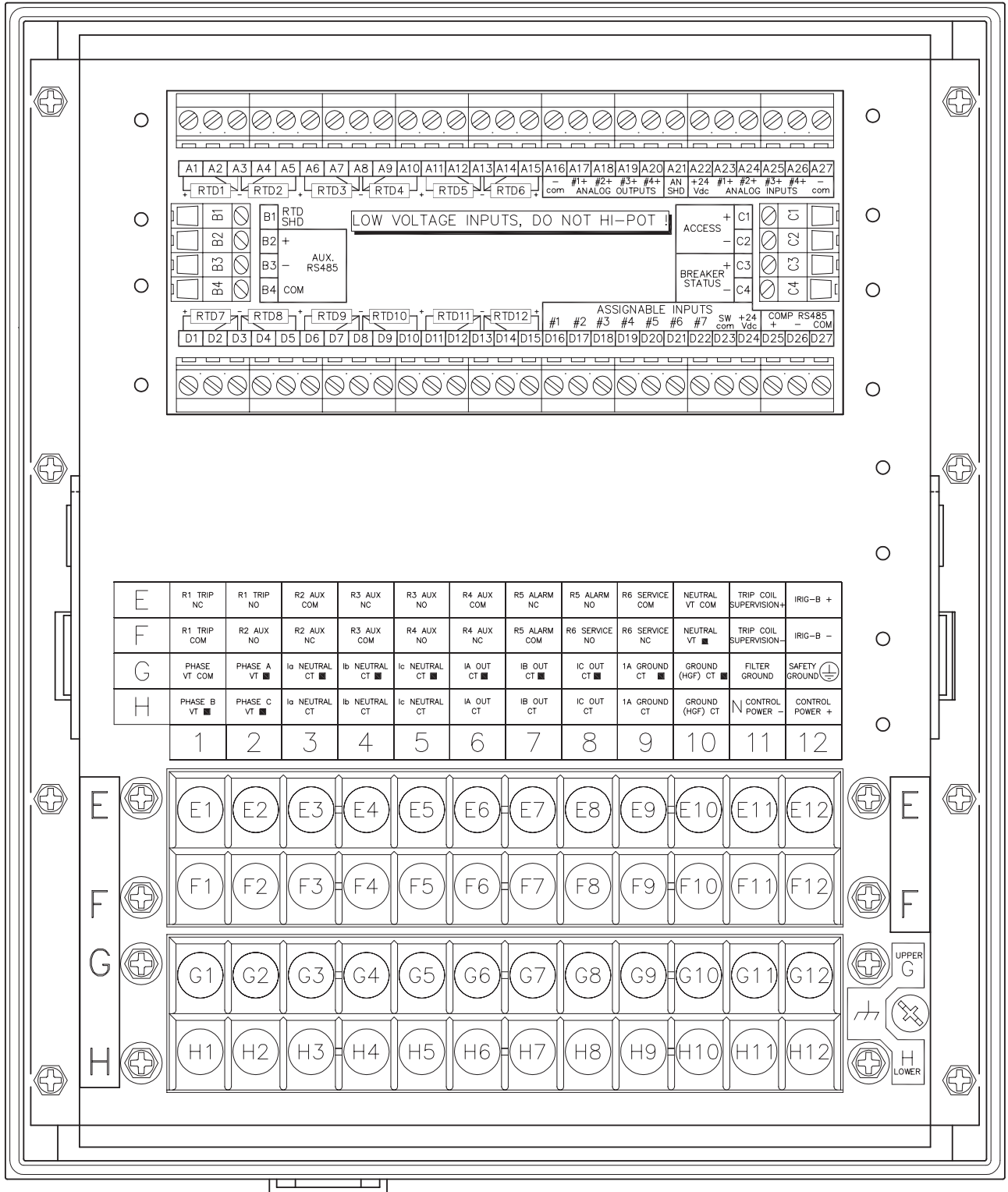
Figure 2-8: TERMINAL LAYOUT
