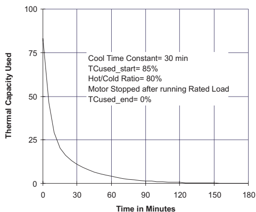
Thermal Model Cooling, Motor Stopped
