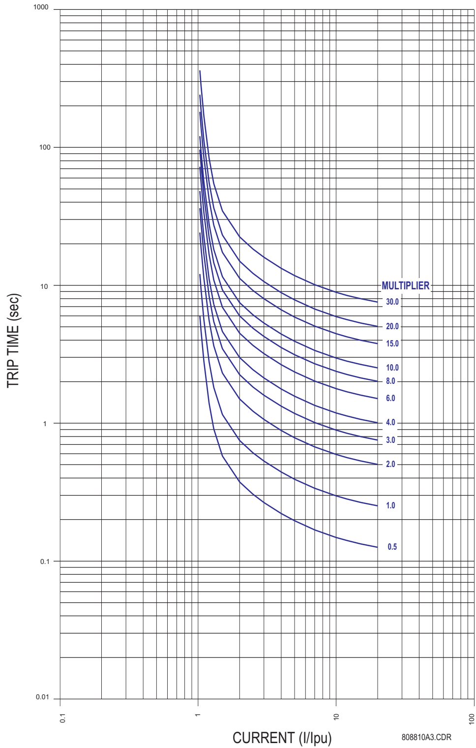
Figure C-7: IAC INVERSE CURVE
