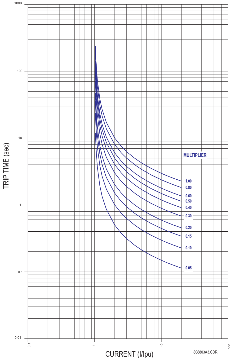
Figure C-10: IEC CURVE A (BS142)
