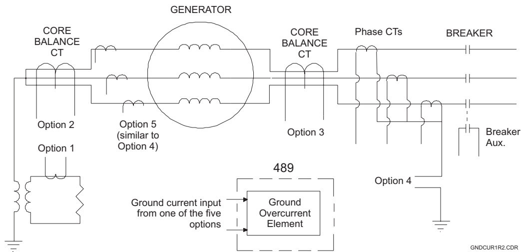
Figure B-3: GROUND OVERCURRENT ELEMENT WITH DIFFERENT CURRENT SOURCE SIGNALS
