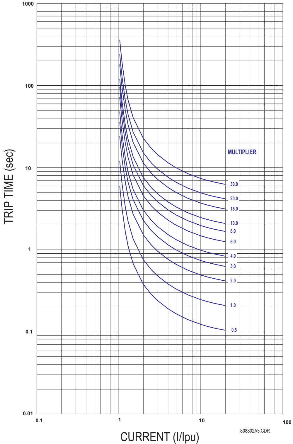
Figure C-1: ANSI MODERATELY INVERSE CURVE
