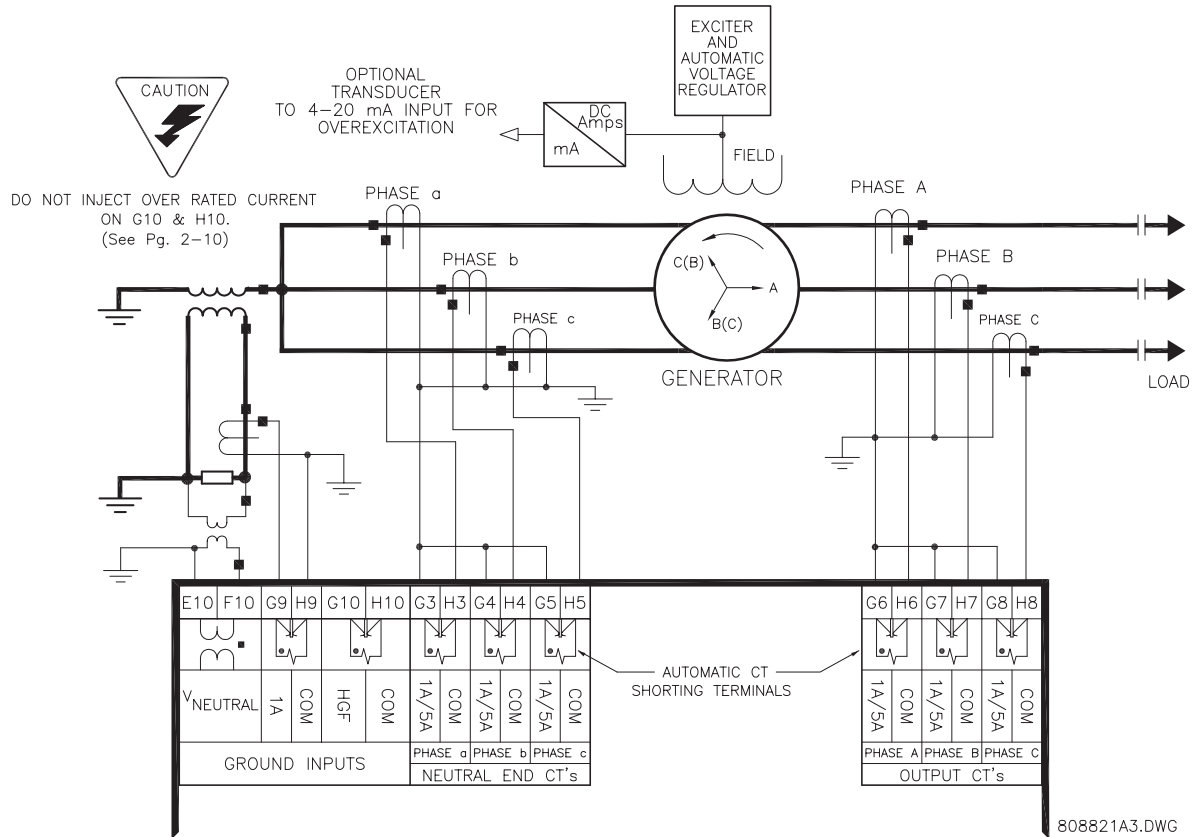
Figure 2-10: TYPICAL WIRING (DETAIL)
