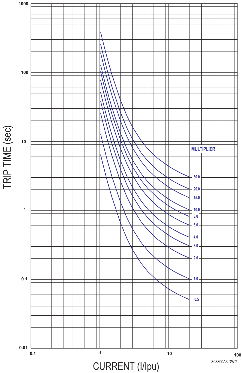
Figure C-3: ANSI VERY INVERSE CURVE
