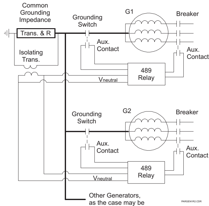
Figure B-2: PARALLEL GENERATORS WITH COMMON GROUNDING IMPEDANCE
