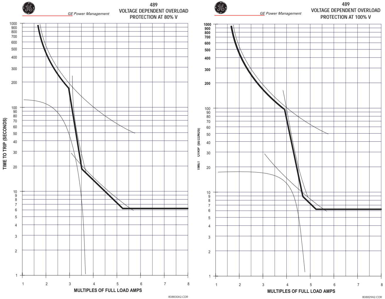
Figure 4-16: VOLTAGE DEPENDENT O/L PROTECTION AT 80% AND 100% VOLTAGE
