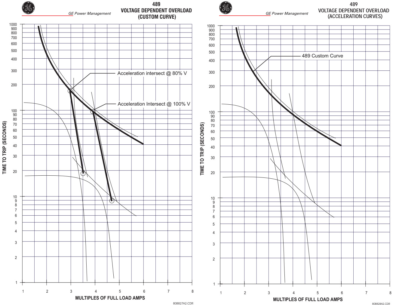
Figure 4–14: VOLTAGE DEPENDENT OVERLOAD CURVES
