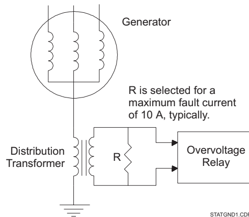
Figure B-1: STATOR GROUND FAULT PROTECTION
