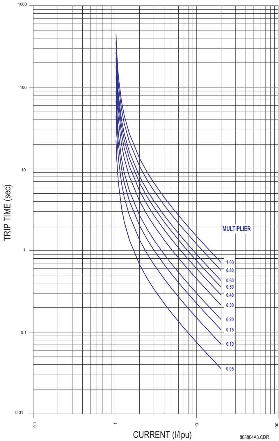
Figure C-11: IEC CURVE B (BS142)
