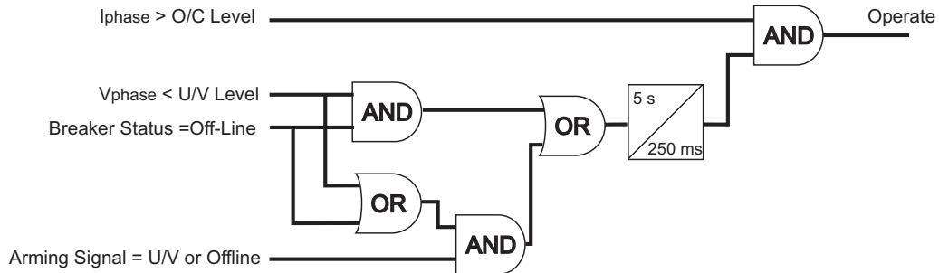
Figure 4–1: INADVERTENT ENERGIZATION
