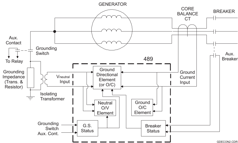
Figure B-4: GROUND DIRECTIONAL ELEMENT CONCEPTUAL ARRANGEMENT
