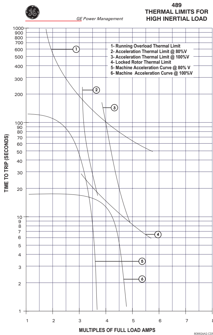
Figure 4-13: THERMAL LIMITS FOR HIGH INERTIAL LOAD
