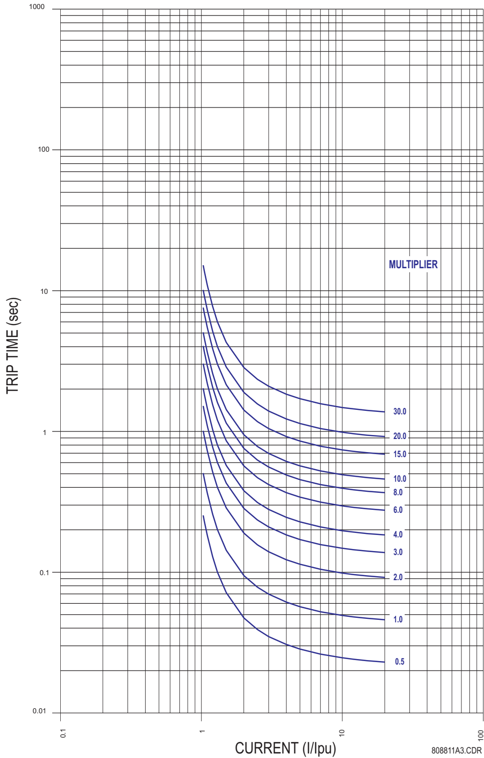
Figure C-6: IAC SHORT INVERSE CURVE
