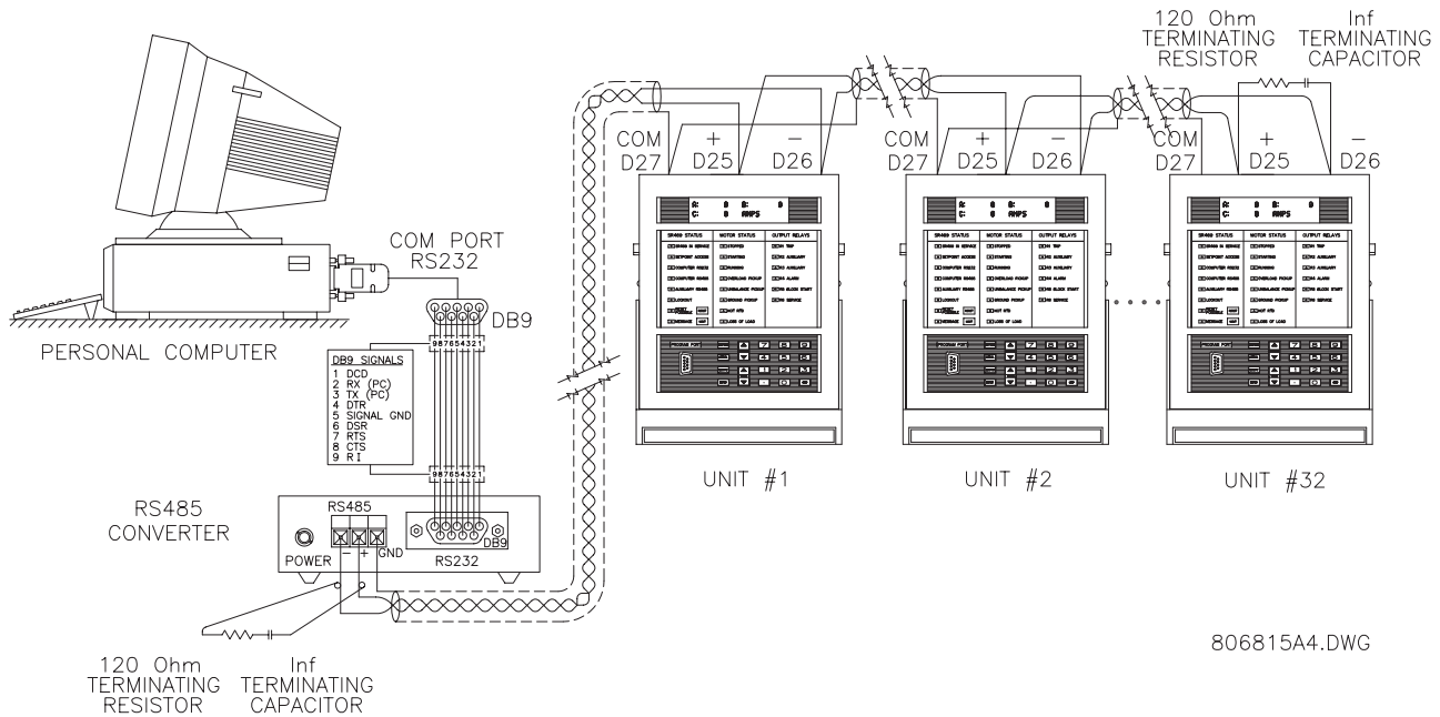
Figure 2-16: RS485 COMMUNICATIONS INTERFACE
