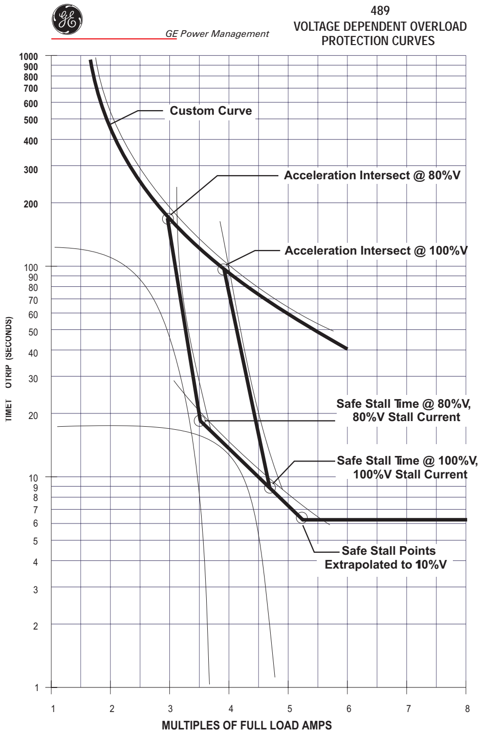
Figure 4-15: VOLTAGE DEPENDENT OVERLOAD PROTECTION CURVES
