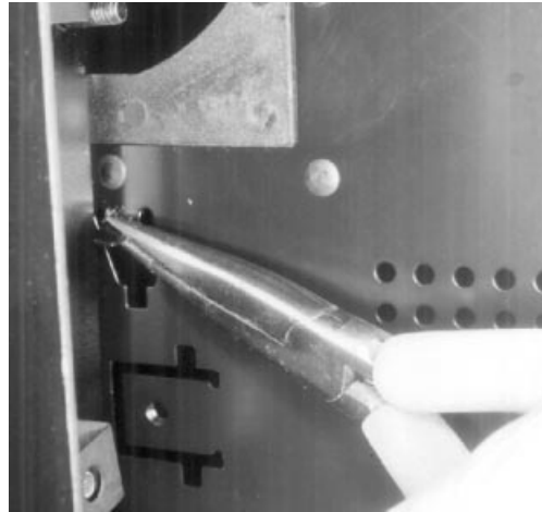
Figure 2–4: BEND UP MOUNTING TABS
