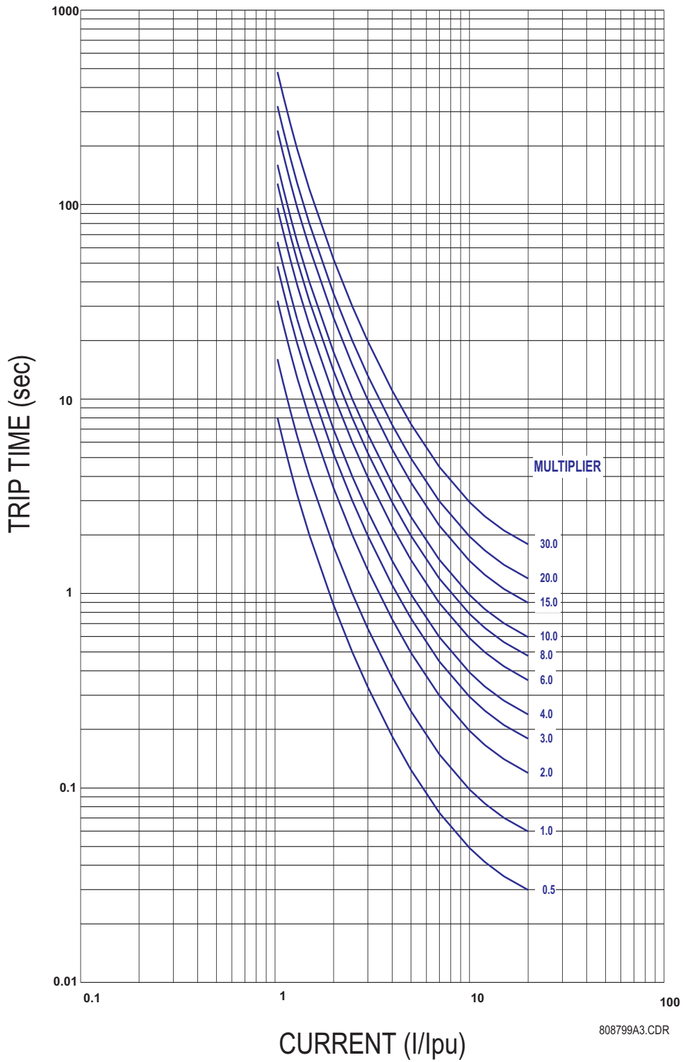
Figure C-4: ANSI EXTREMELY INVERSE CURVE
