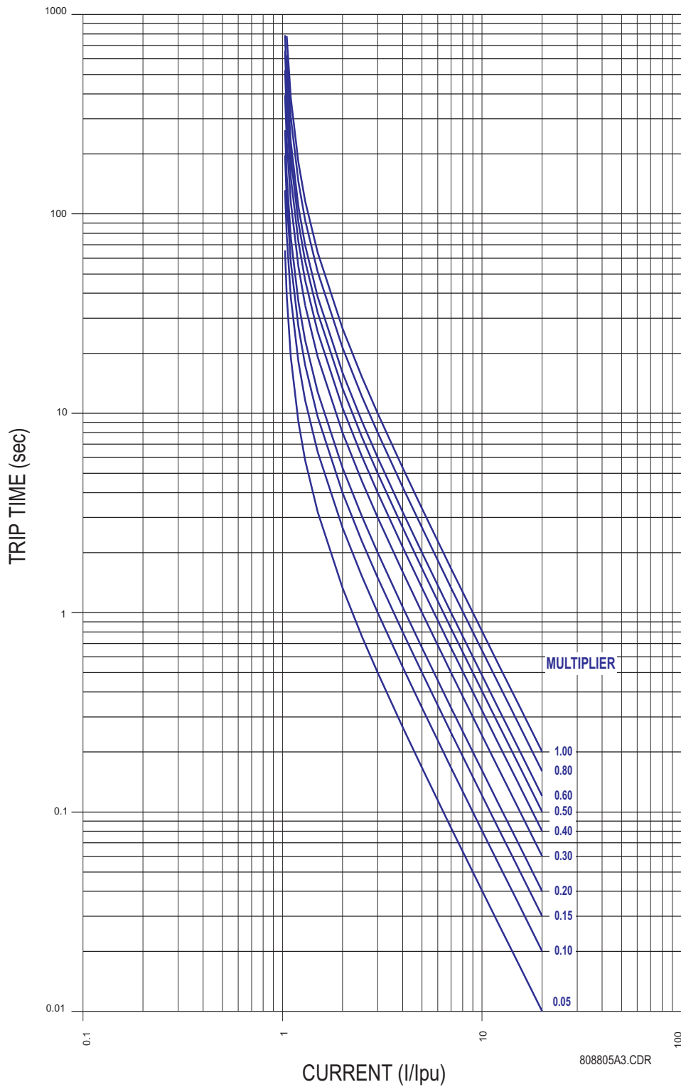
Figure C-12: IEC CURVE C (BS142)
