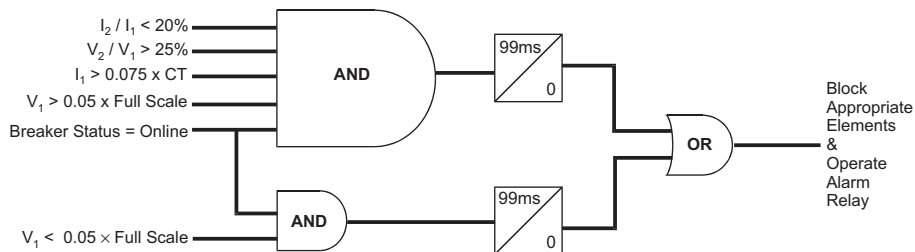
Figure 4-20: VT FUSE FAILURE
