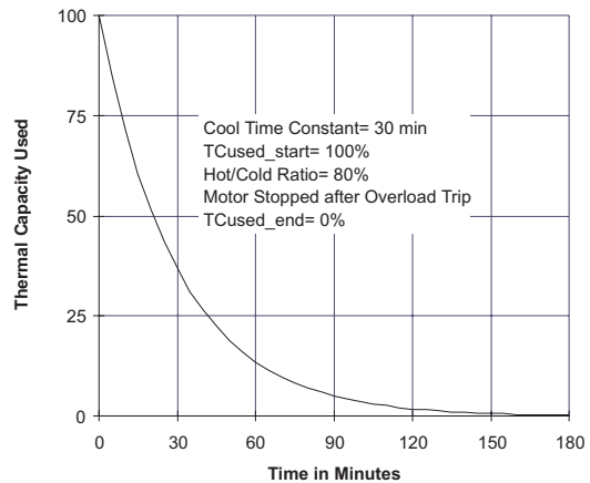
Thermal Model Cooling, Motor Tripped
