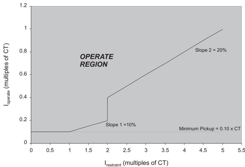
Figure 4-4: DIFFERENTIAL ELEMENTS
