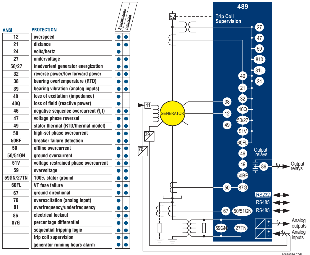
Figure 1-1: SINGLE LINE DIAGRAM
