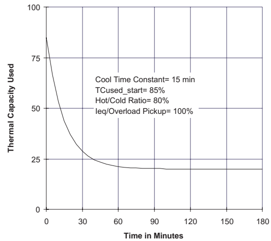
Thermal Model Cooling, 100% Load
