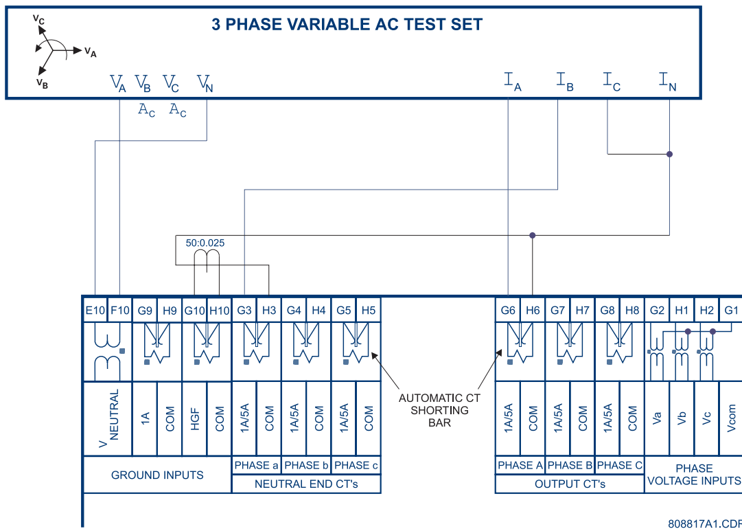
Figure 7–2: SECONDARY INJECTION SETUP #2
