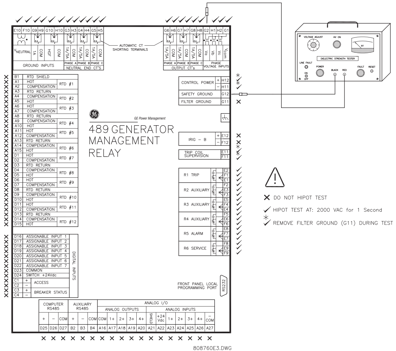
Figure 2-17: TESTING THE 489 FOR DIELECTRIC STRENGTH
