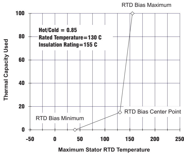
Figure 4-18: RTD BIAS CURVE
