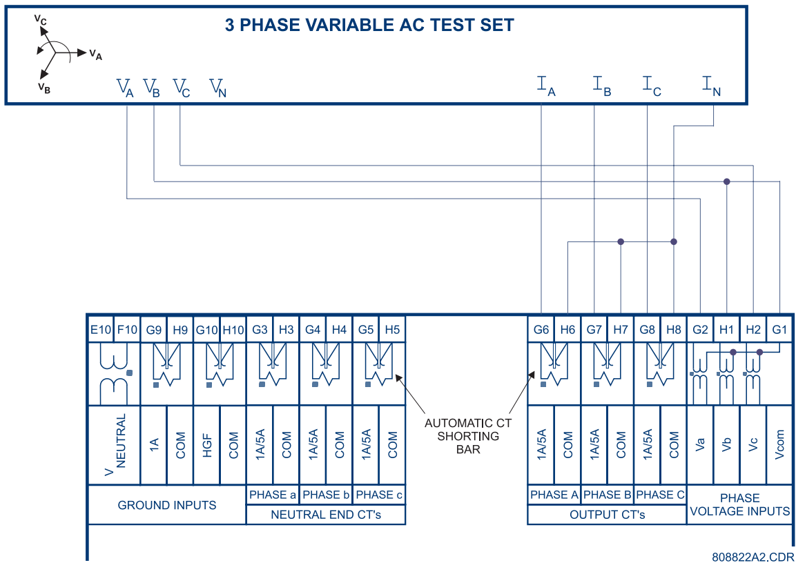
Figure 7-4: SECONDARY INJECTION TEST SETUP #3
