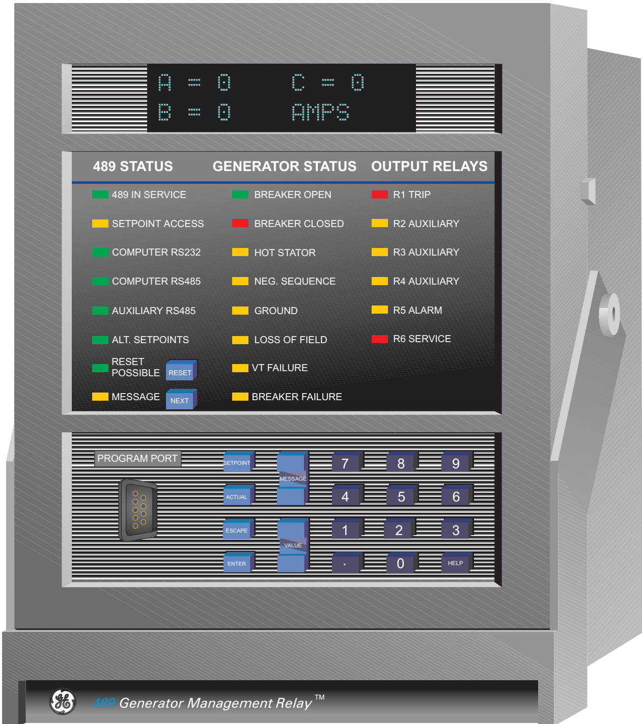
Figure 3–1: 489 FACEPLATE
