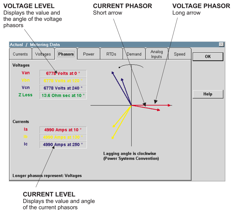
Figure 8-7: PHASORS
