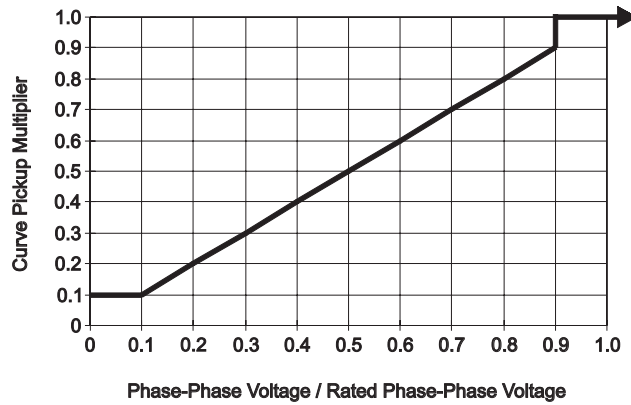
Figure 4-2: VOLTAGE RESTRAINT CHARACTERISTIC
