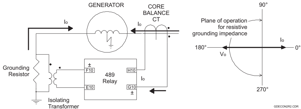
Figure B-5: GROUND DIRECTIONAL ELEMENT POLARITIES AND PLANE OF OPERATION
