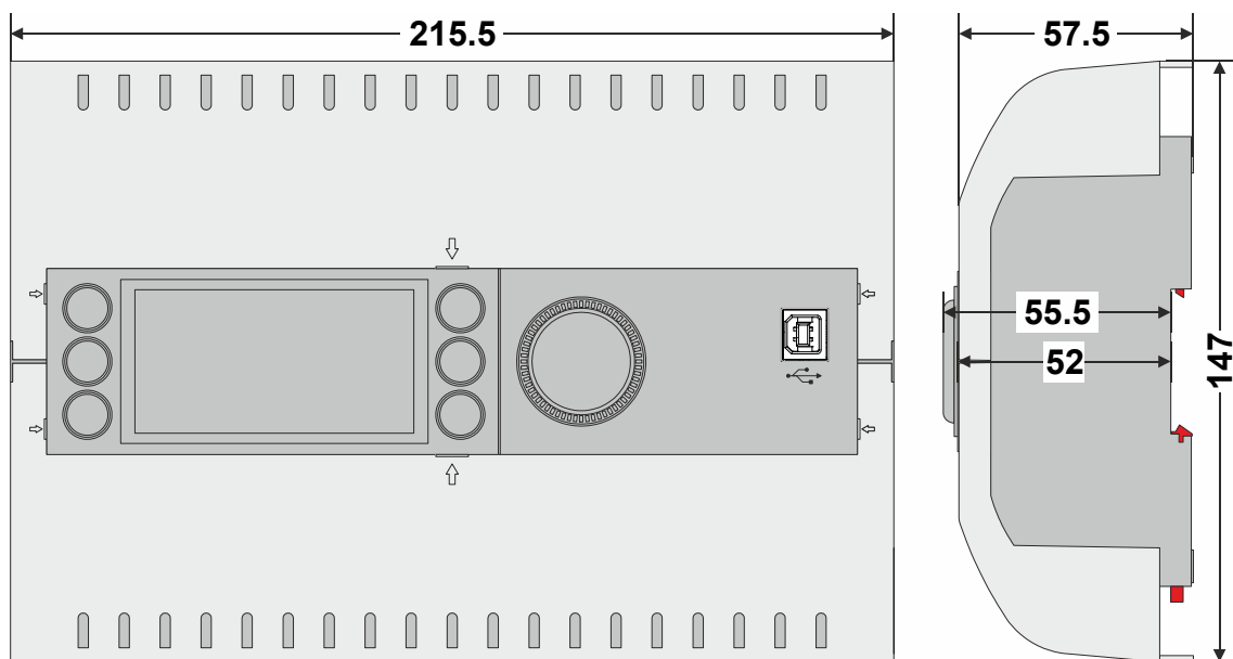
Fig. 11. Excel Web II Controller with built-in HMI (with MVC-80-AC1), dimensions (in mm)
