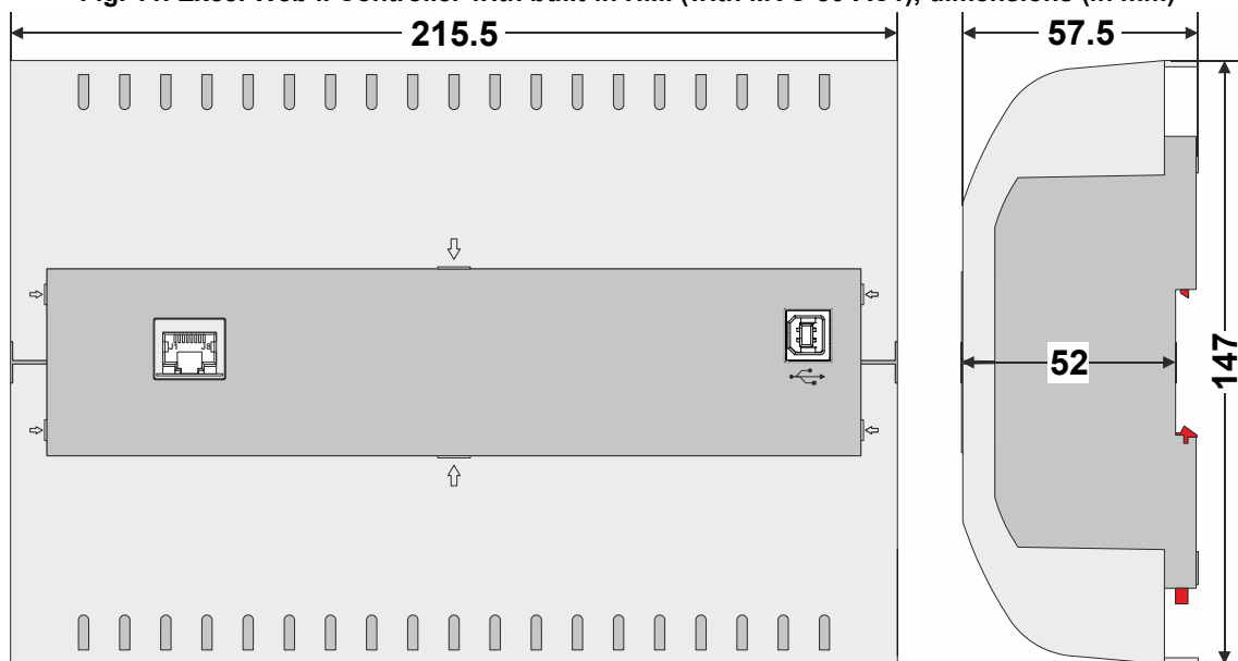
Fig. 12. Excel Web II Controller with RJ45 socket for XL2000HMI-A External HMI (with MVC-80-AC1), dimensions (in mm)
